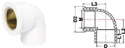
Female Elbow (Brass)
