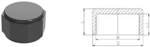
Cap (Thread)
