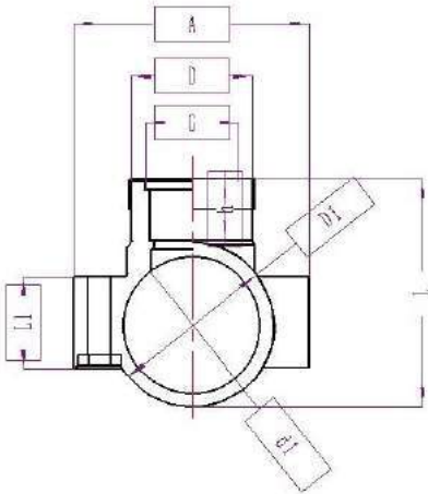
PP Clamp Saddle
