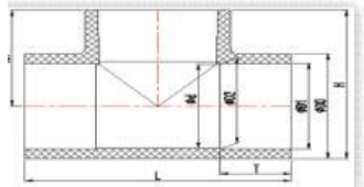
PVC Equal Tee
