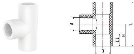
Female Tee
