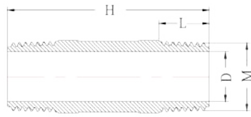
Nipple
