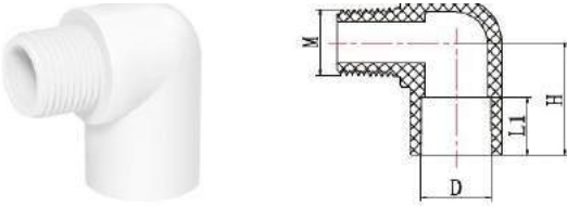
Male Elbow
