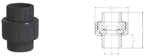
UNION
