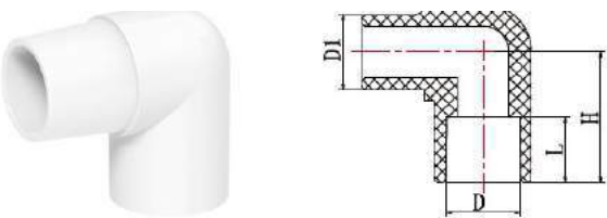
Street Elbow
