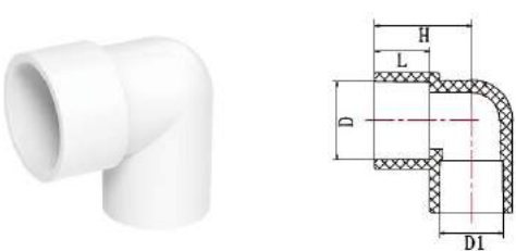
Reducing Elbow
