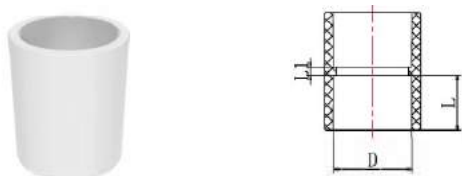
Coupling
