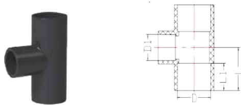
REDUCING TEE
