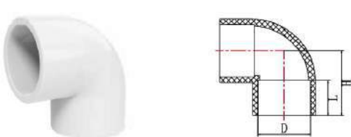
90 Deg Elbow
