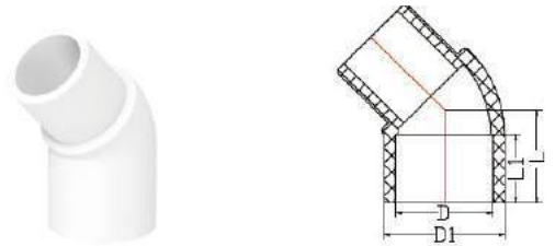
45 Deg Street Elbow
