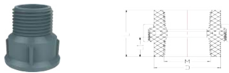
Male Socket
