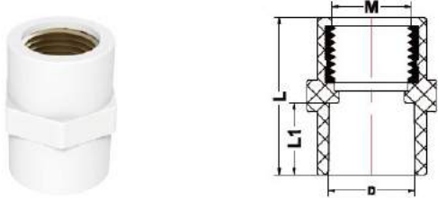
Female Adapter (Brass)
