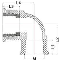
90 Deg Elbow (Brass) II
