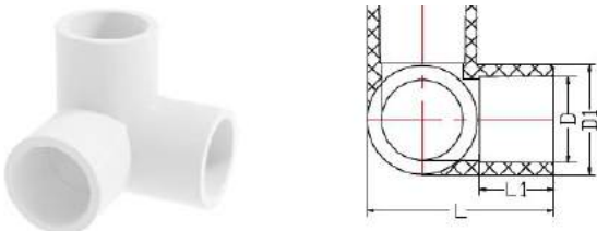
Side Outlet Elbow
