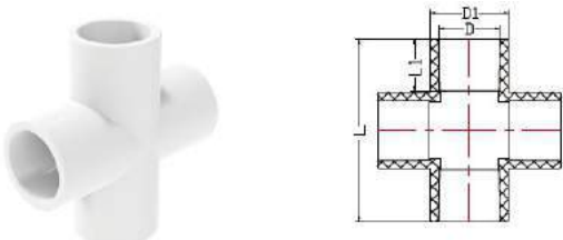
Cross
