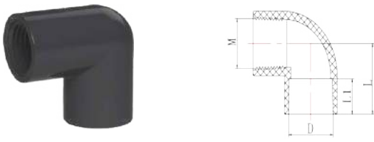
Female Elbow
