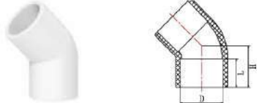
45 Deg Elbow
