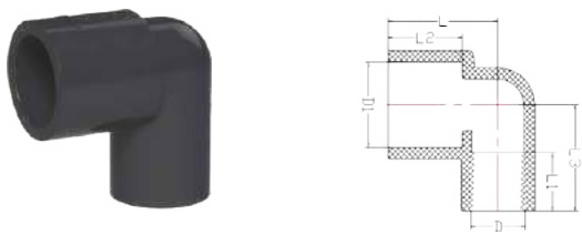
Reducing Female Elbow
