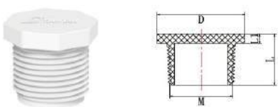
Male Plug
