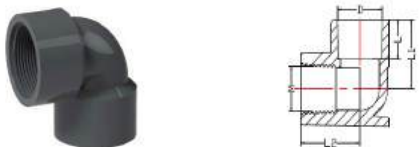
Female Elbow
